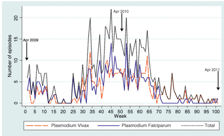
FIGURE 3. Sequence chart of Plasmodium falciparum , Plasmodium vivax , and total episodes over 101 weeks of observation, Chano Mille Kebele, south Ethiopia, 2009–2011. This figure appears in color at www.ajtmh.org .
