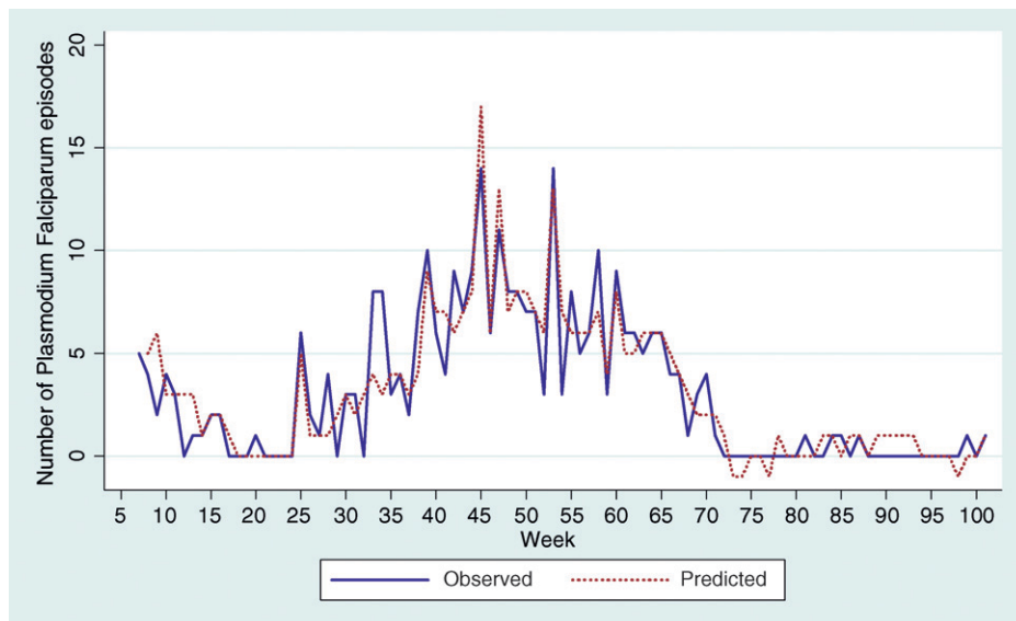
FIGURE 5. Actual and model-predicted Plasmodium falciparum episodes over 95 weeks of observation, Chano Mille Kebele, south Ethiopia, 2009–2011. This figure appears in color at www.ajtmh.org .
